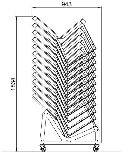
SIDE VIEW ON SEATING STORAGE
