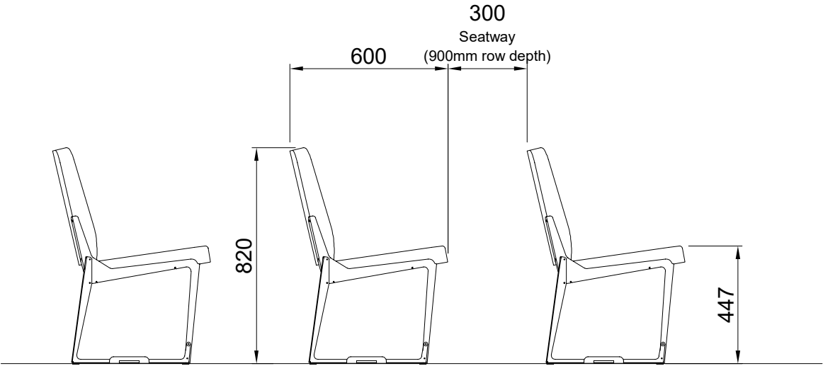
SIDE VIEW ON SEATING
